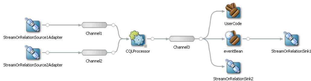
Figure 1–1 Oracle Event Processing Application
