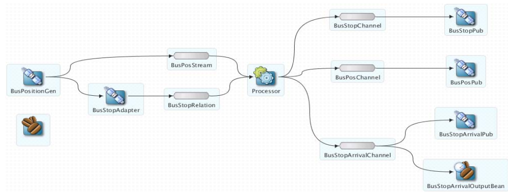
Figure 7-4 Oracle Spatial Example Event Processing Network
