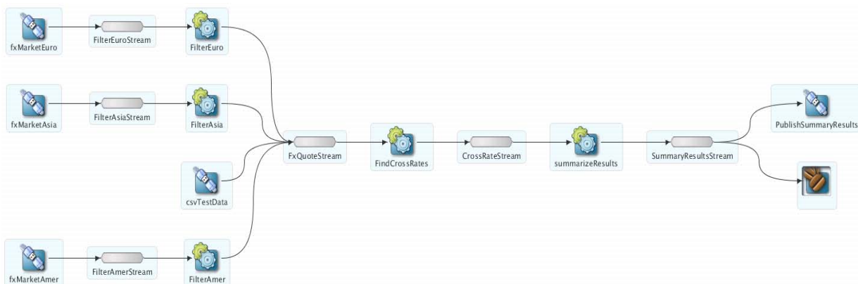
Figure 7-5 FX Example Event Processing Network
